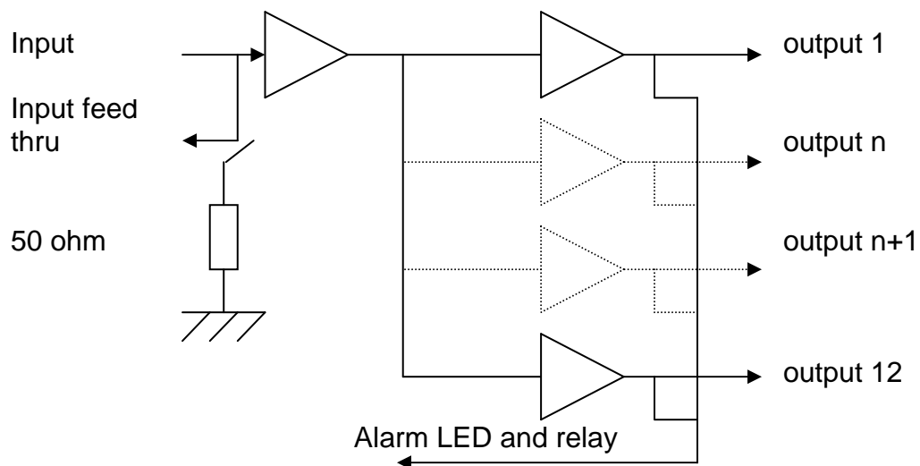
Figure 1. ptf 1205 Schematic
