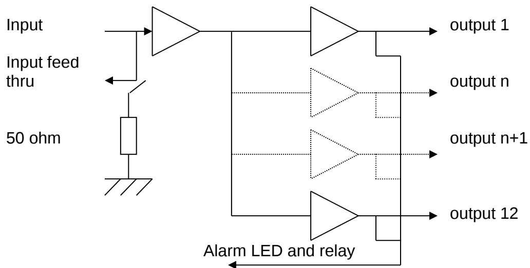
Figure 1. ptf 1203 Schematic
